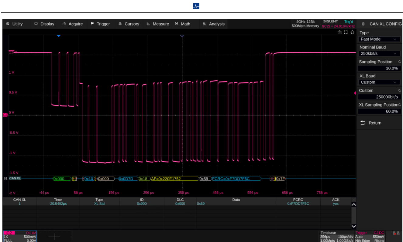
Figure 5 Protocol signal settings for CAN XL Fast mode
