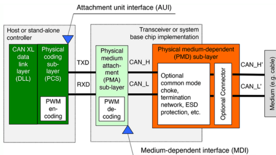
Figure 1 CAN Protocol Underlying Implementation
