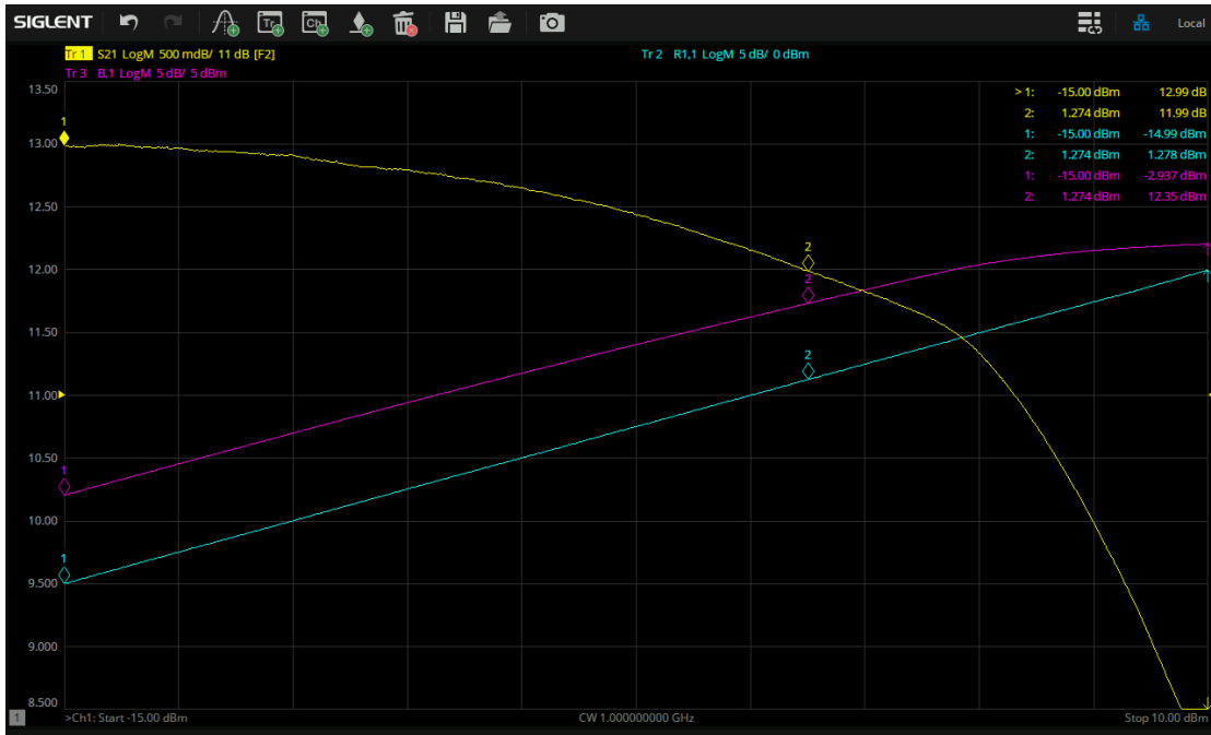
Figure 4-4 Test result of amplifier with power sweep
