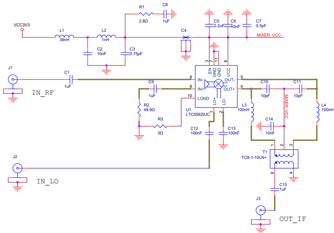
Figure 3-3 Mixer module schematic diagram
