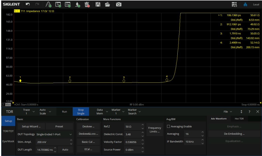
Figure 4-15 TDR test result of long through line
