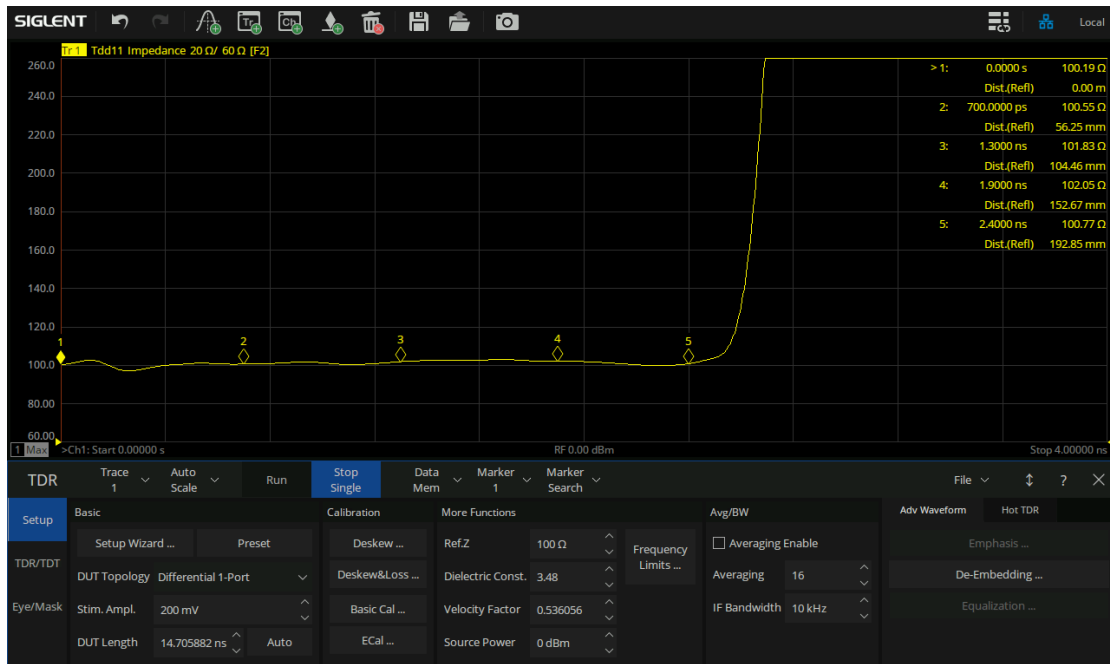
Figure 4-19 TDR test result of differential line
