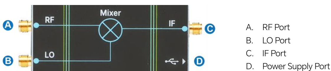
Figure 3-2 Schematic diagram of mixer module
