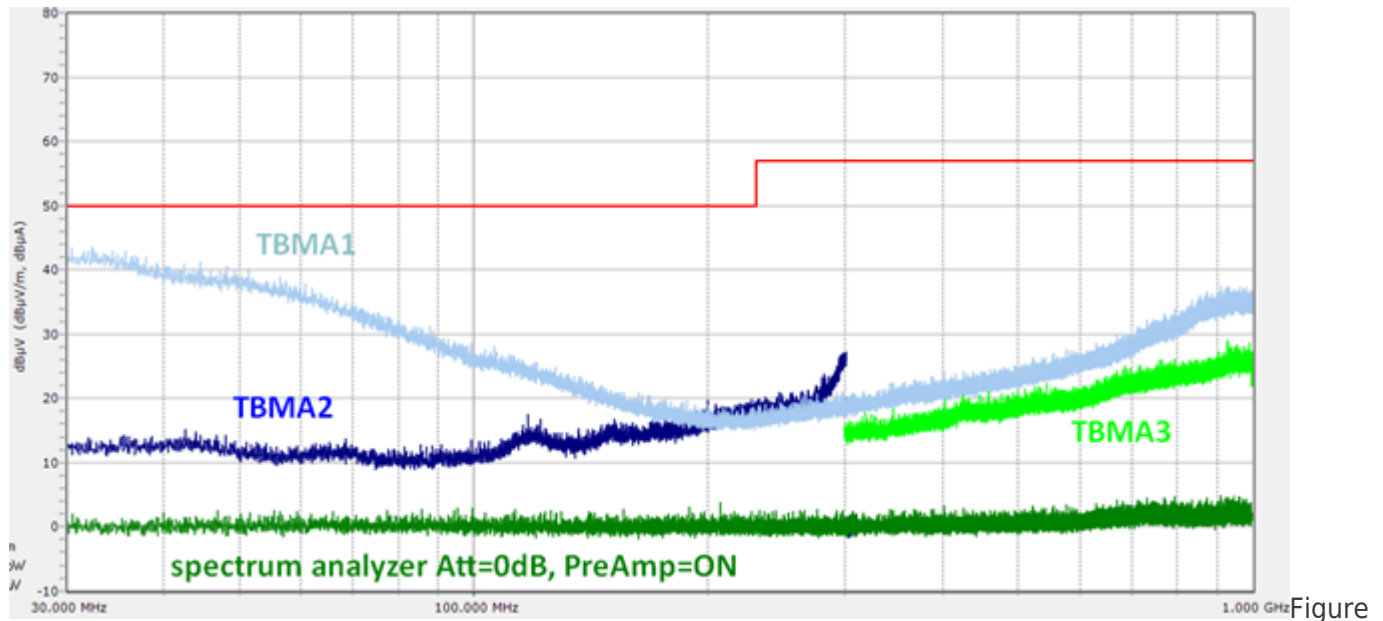
15: CISPR32 Class A radiated emissions for various antennas
