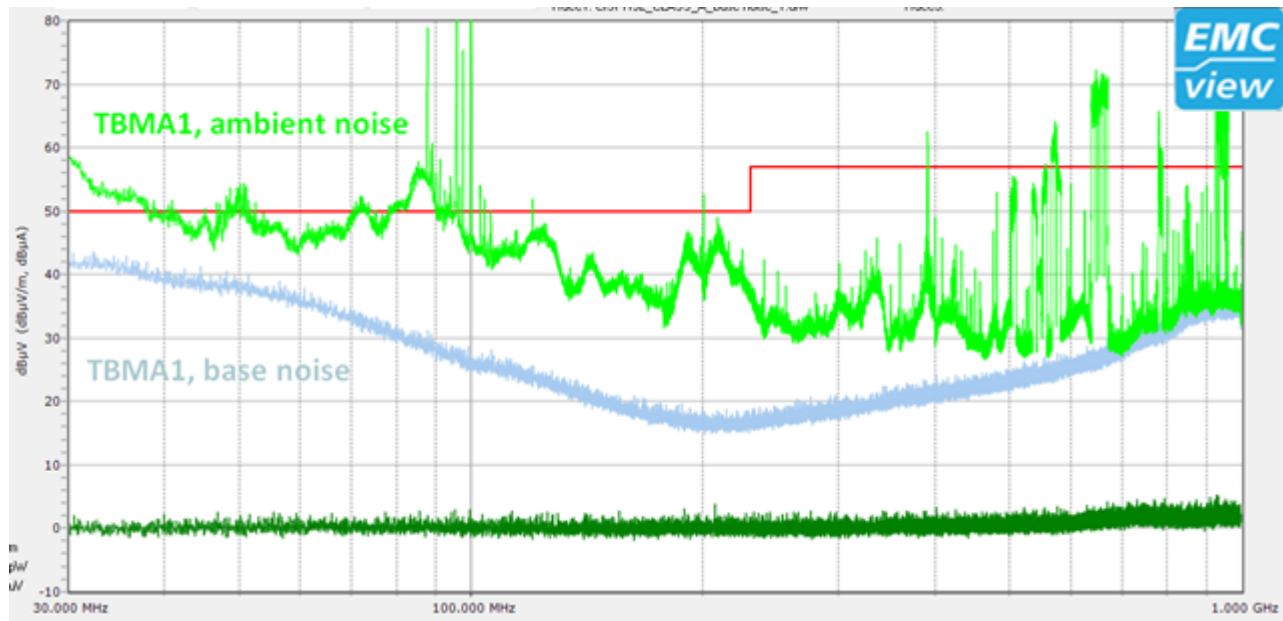
16: Example of ambient scan in an industrial environment
