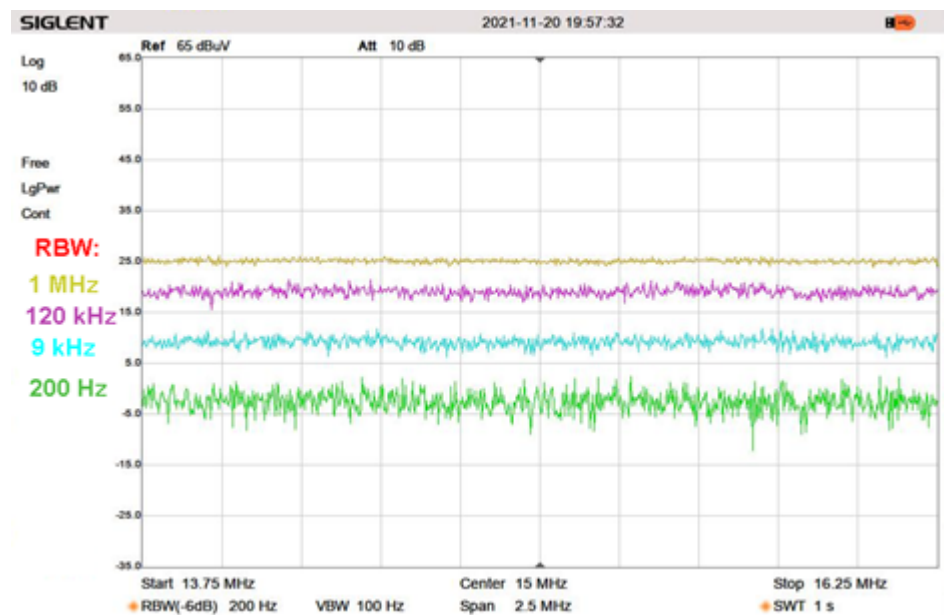
Figure 3: Spectrum analyzer DANL level versus resolution bandwidth.
