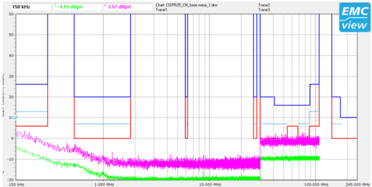
Figure 14: CISPR 25 Class 5 TEM example
