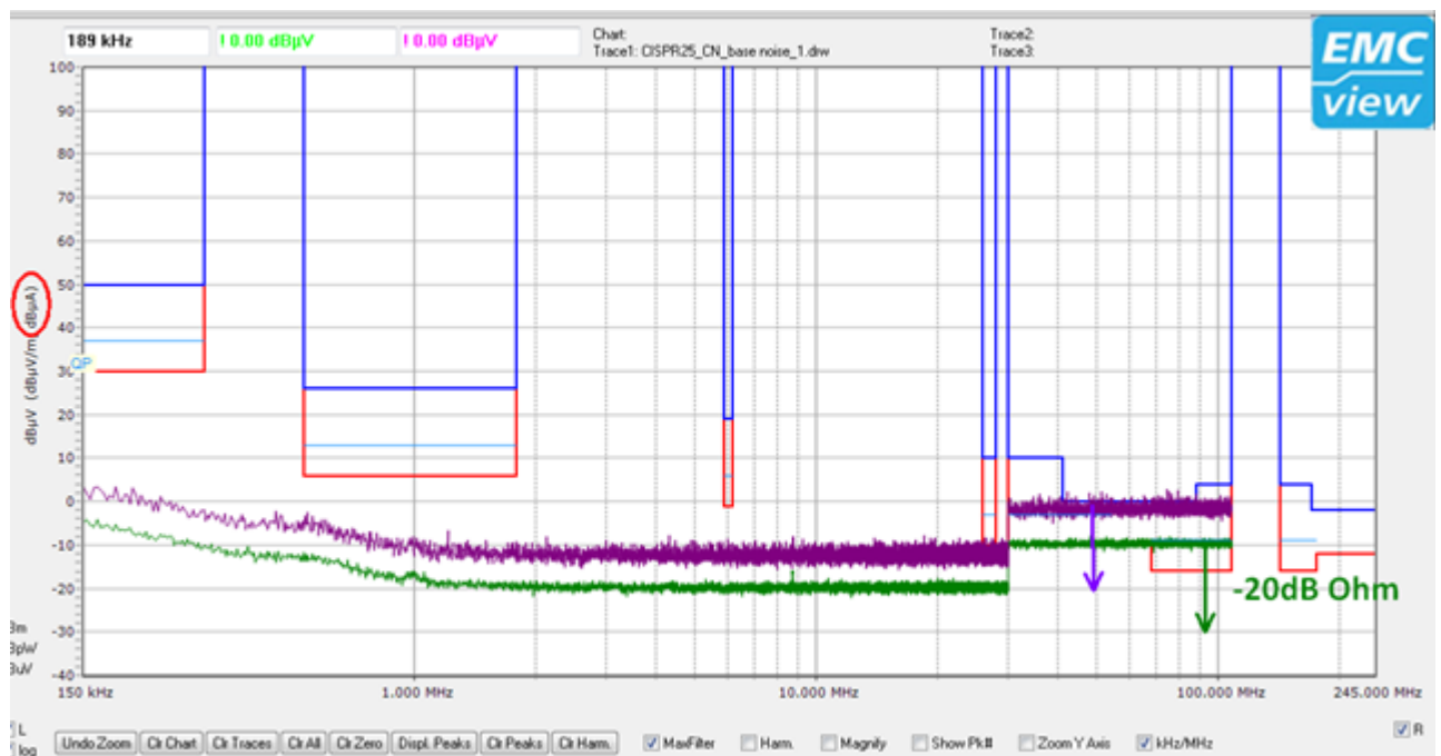
Figure 12: Example of CISPR 25 Class 5 Current Method.
