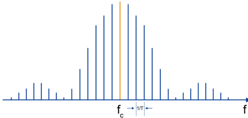
Figure 2-2 spectrum of radio frequency pulse signal
